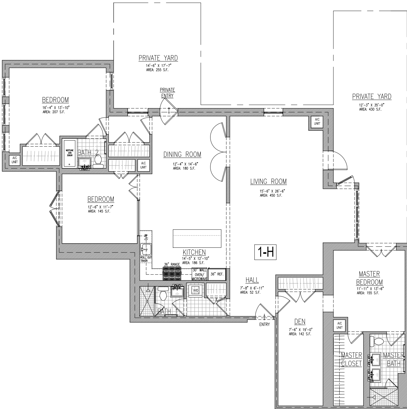
FIRST FLOOR: 2,160 SQ.FT. - KEY PLAN
